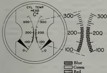
FIGURE 10-29. Cylinder head temperature gage.
